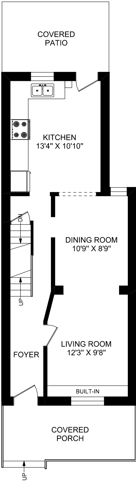
MAIN FLOOR 604 SQUARE FEET (CEILING HEIGHT : 9' -0")
