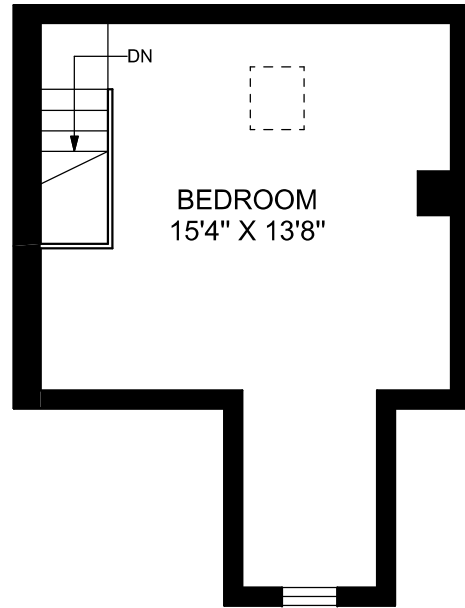
THIRD FLOOR 304 SQUARE FEET (CEILING HEIGHT : 8'-0")
