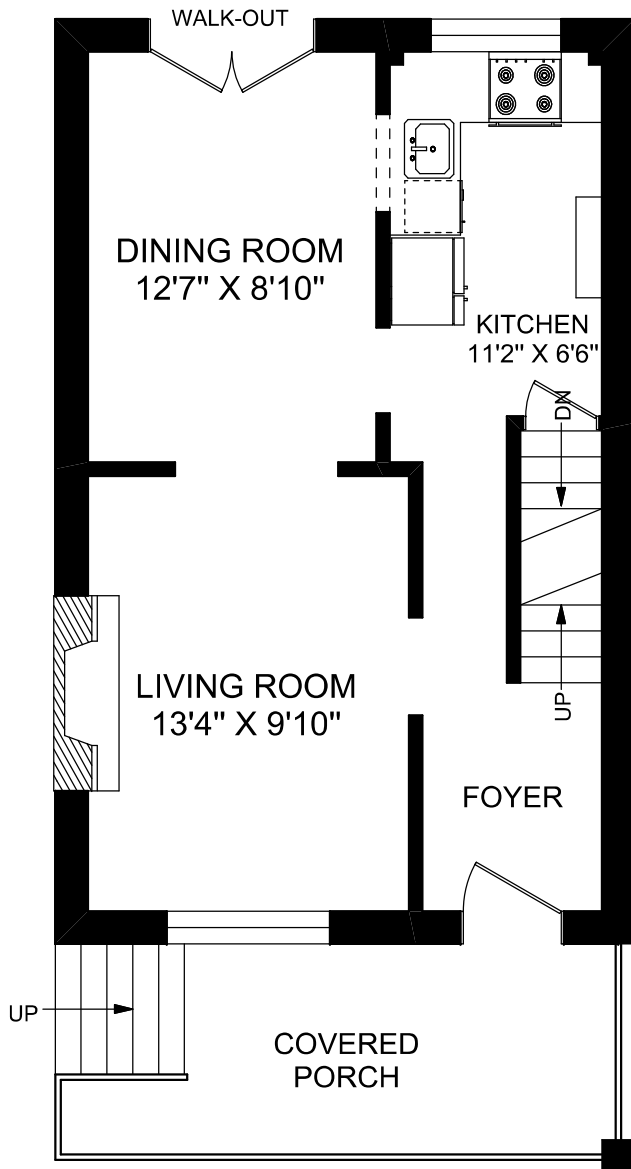
MAIN FLOOR 505 SQUARE FEET
