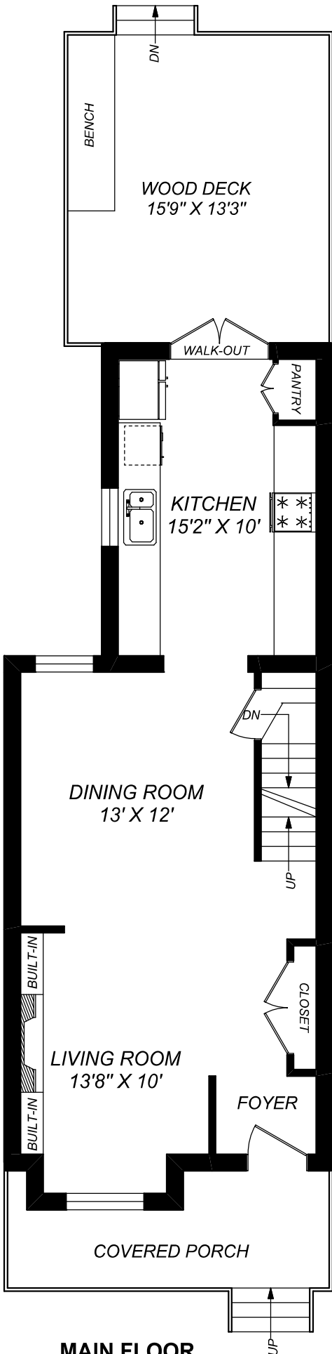
MAIN FLOOR 646 SQUARE FEET (CEILING HEIGHT : 9'-4")
