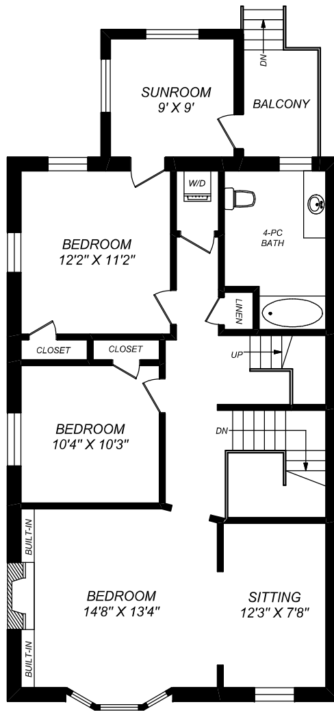
SECOND FLOOR 1103 SQUARE FEET (CEILING HEIGHT : 8'-0")
